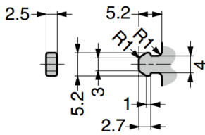
Counter plate head details
